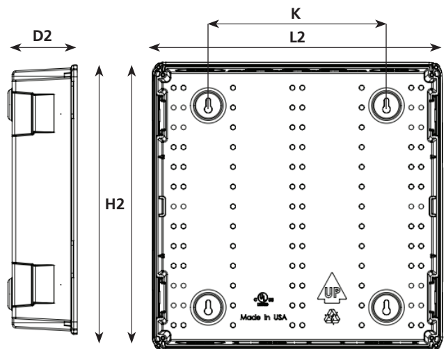
Flush Mounted Enclosure
